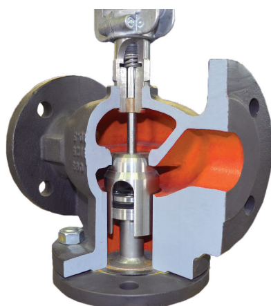
Sectional view of bælz 340-2-B-EMF plug
